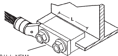
Wide Flange Beams (Flange Parallel) use YGIBW
