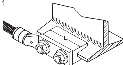
Standard Beams (Flange Angled) use YGIBS
