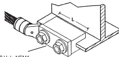
2 Hole NEMA Spacing Wide Flange Beams (Flange Parallel) use YGIBW
