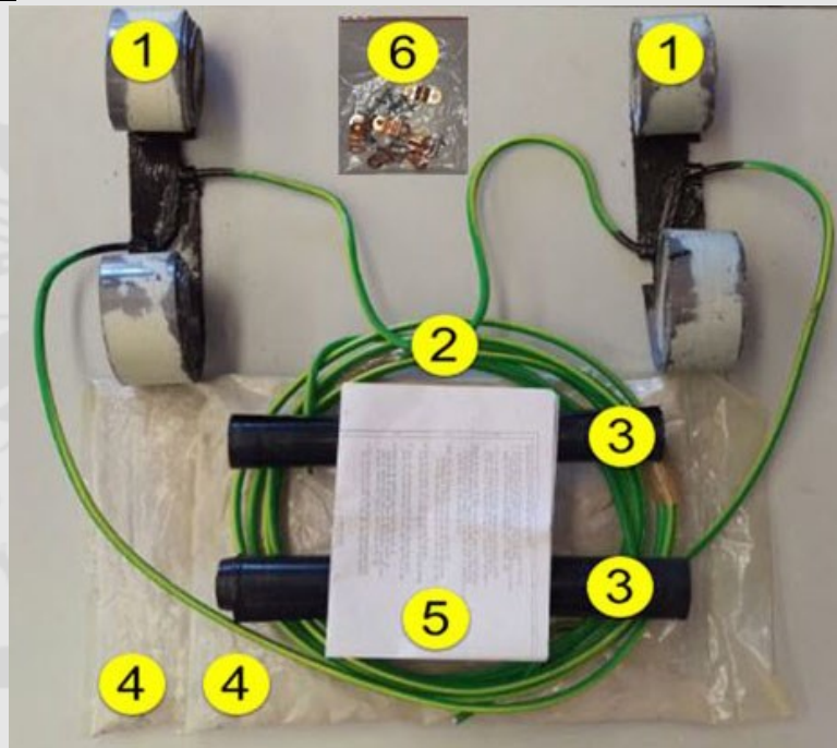
TM11728—EARTH MANHOLE LEAD—TELSTA
