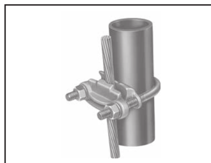
Wire Parallel to Pipe
