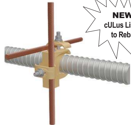
Rebar Connection
