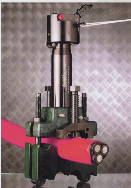
Standard Cable Spiker with Spiking Jack
